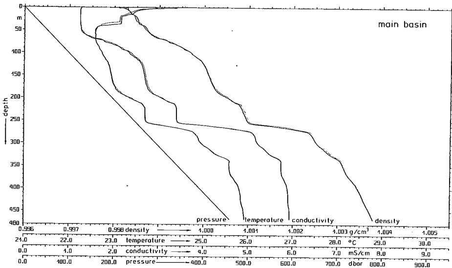
Fig. 2: Vertical profiles of the in-situ density, temperature, conductivity, and pressure (location 9, profile U 35; 23 January 1975); — = lowering, — = lifting of the underwater probe.
