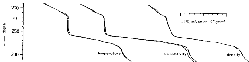
Fig. 4: Fine structure of the distribution of parameters within the layer with the largest gradient (location 5, profile U5; 5 Dez. 1974); - = lowering, - = lifting of the underwater probe.
